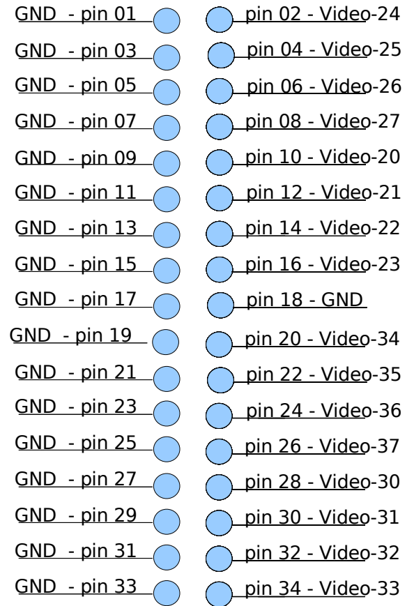
MDVA 3000 On-board Video Connector
