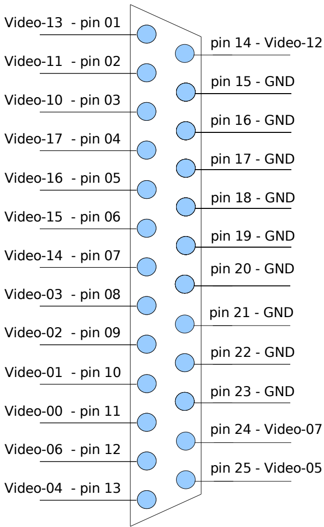
MDVA 3000 Front Panel Video Connector
